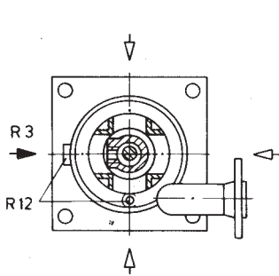
Stuffing boxes P12 and P02
